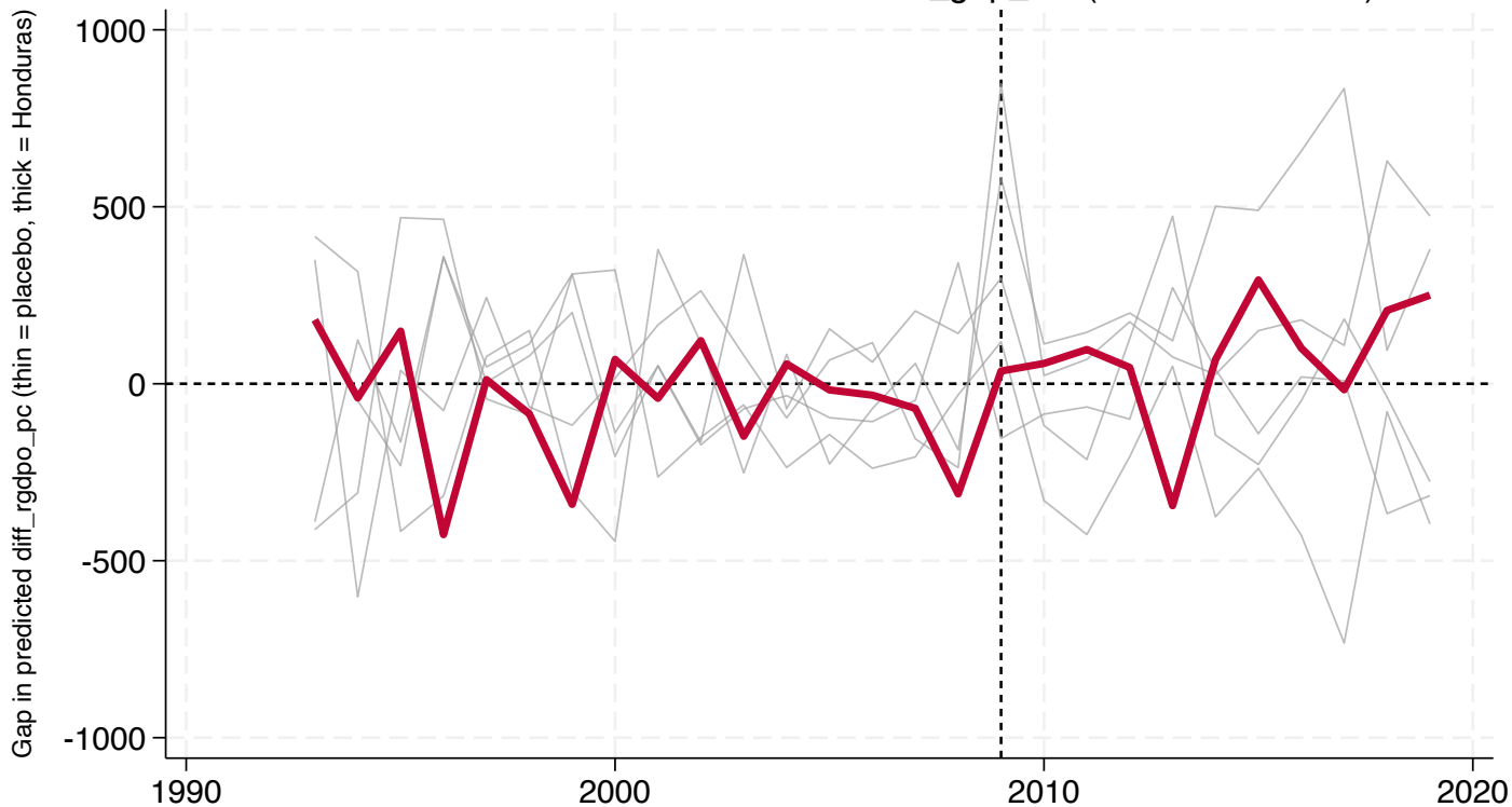
Central America & the Caribbean: factors_gdp_diff (outliers excluded)
